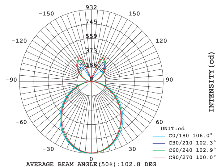
LUMINOUS INTENSITY DISTRIBUTION
